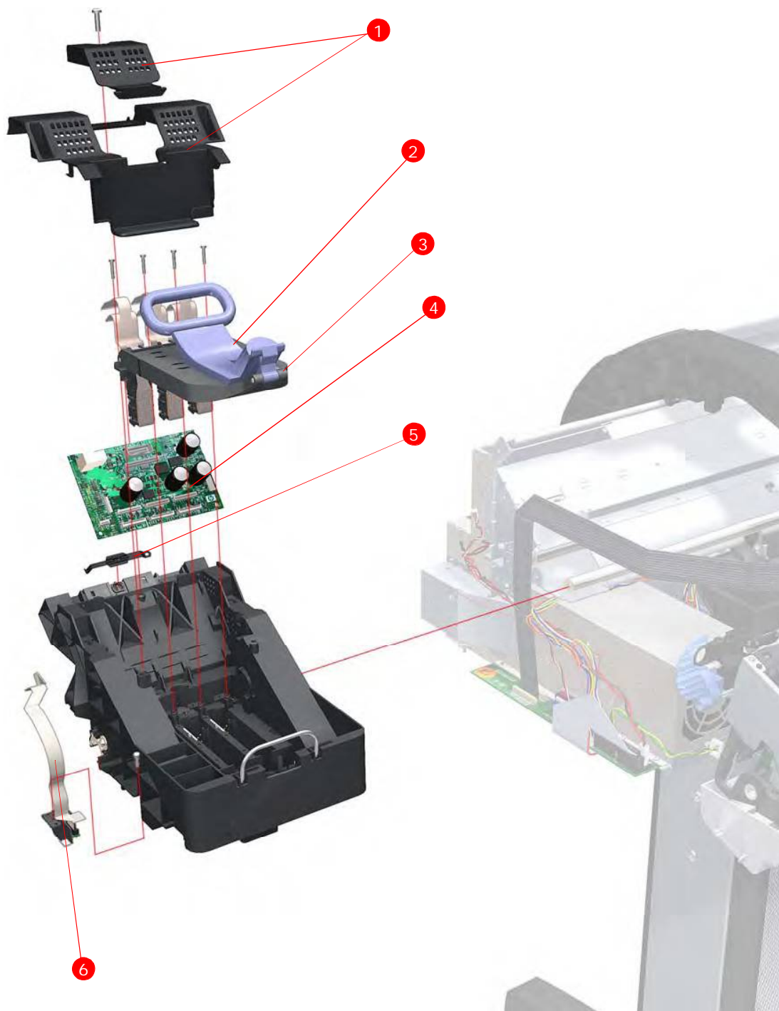
Figure 5-9: Carriage Assembly (T1120/T1120ps/T620)
